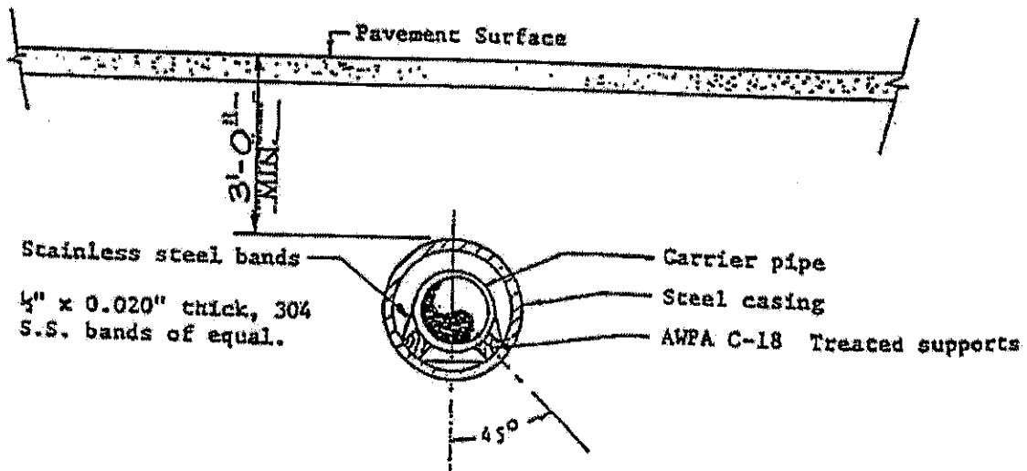
Typical Bored Casing Detail
